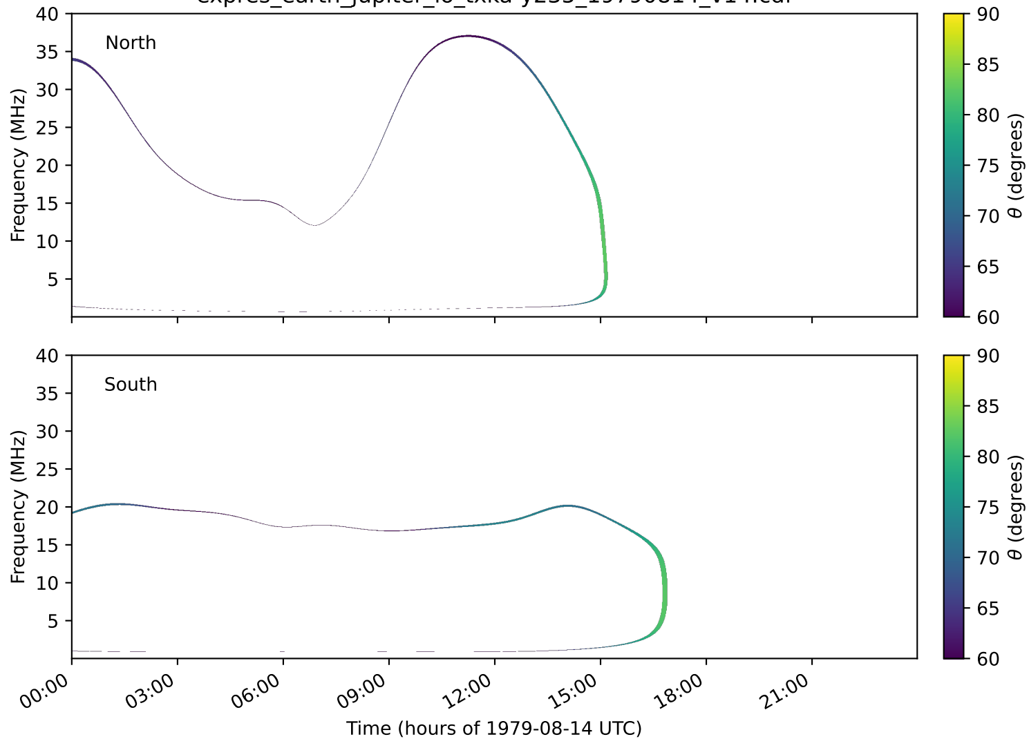
expres_earth_jupiter_io_txka-y235_19790814_v14.cdf
