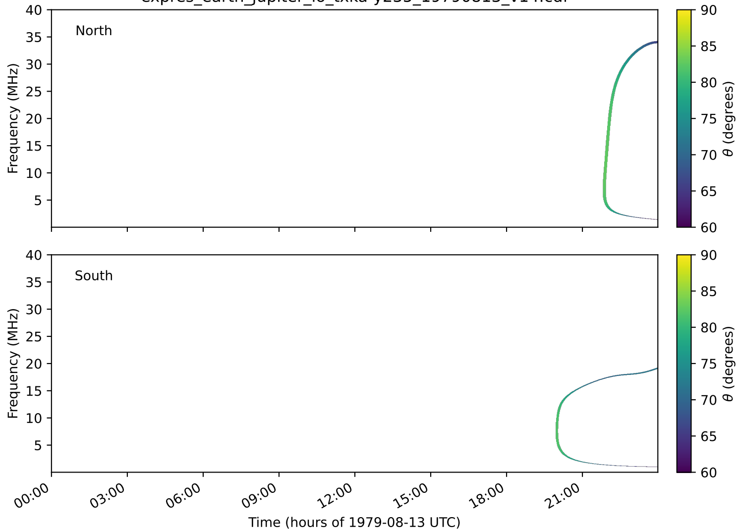
expres_earth_jupiter_io_txka-y235_19790813_v14.cdf
