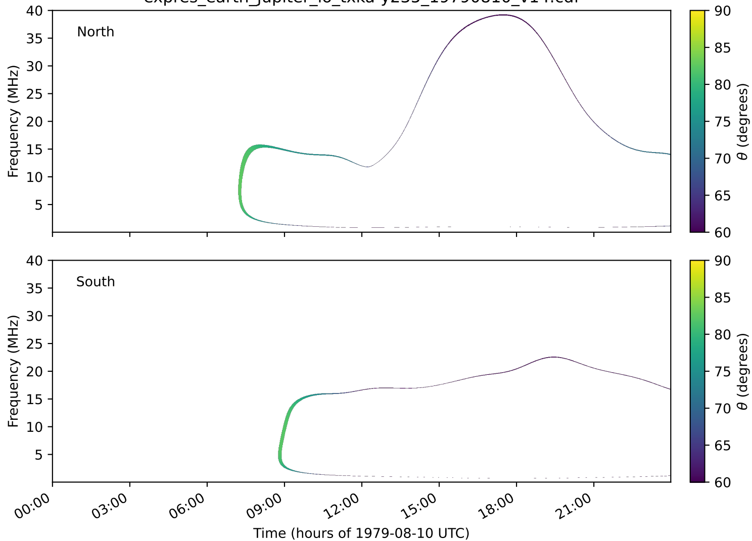
expres_earth_jupiter_io_txka-y235_19790810_v14.cdf
