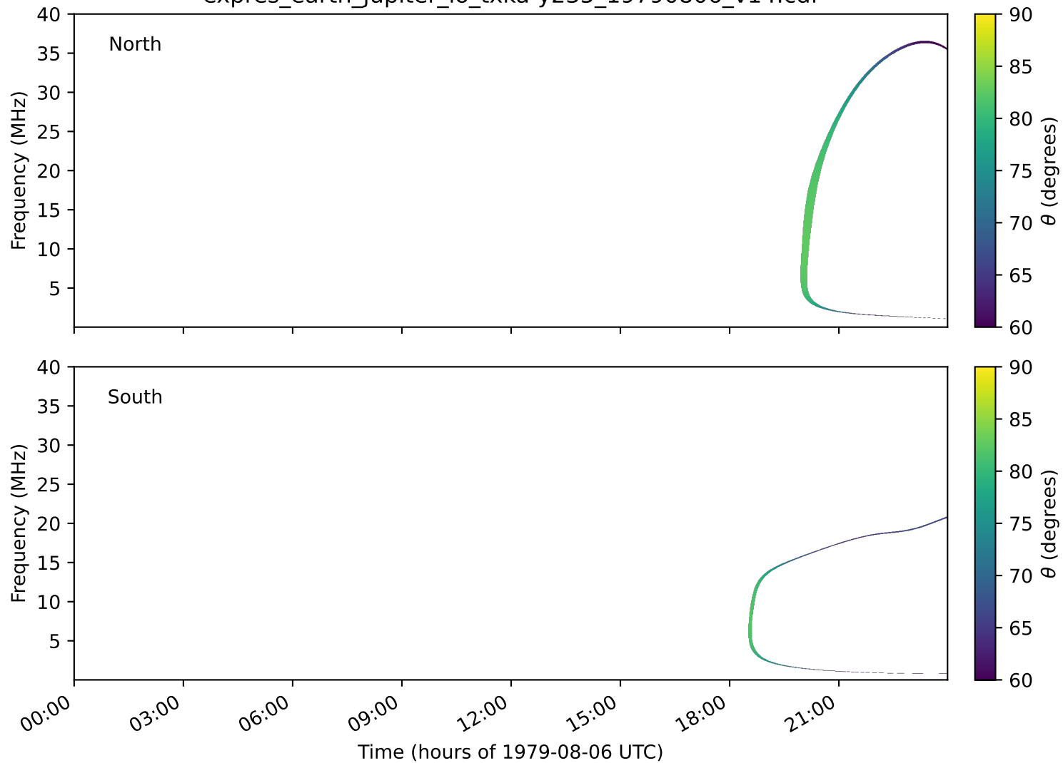
expres_earth_jupiter_io_txka-y235_19790806_v14.cdf
