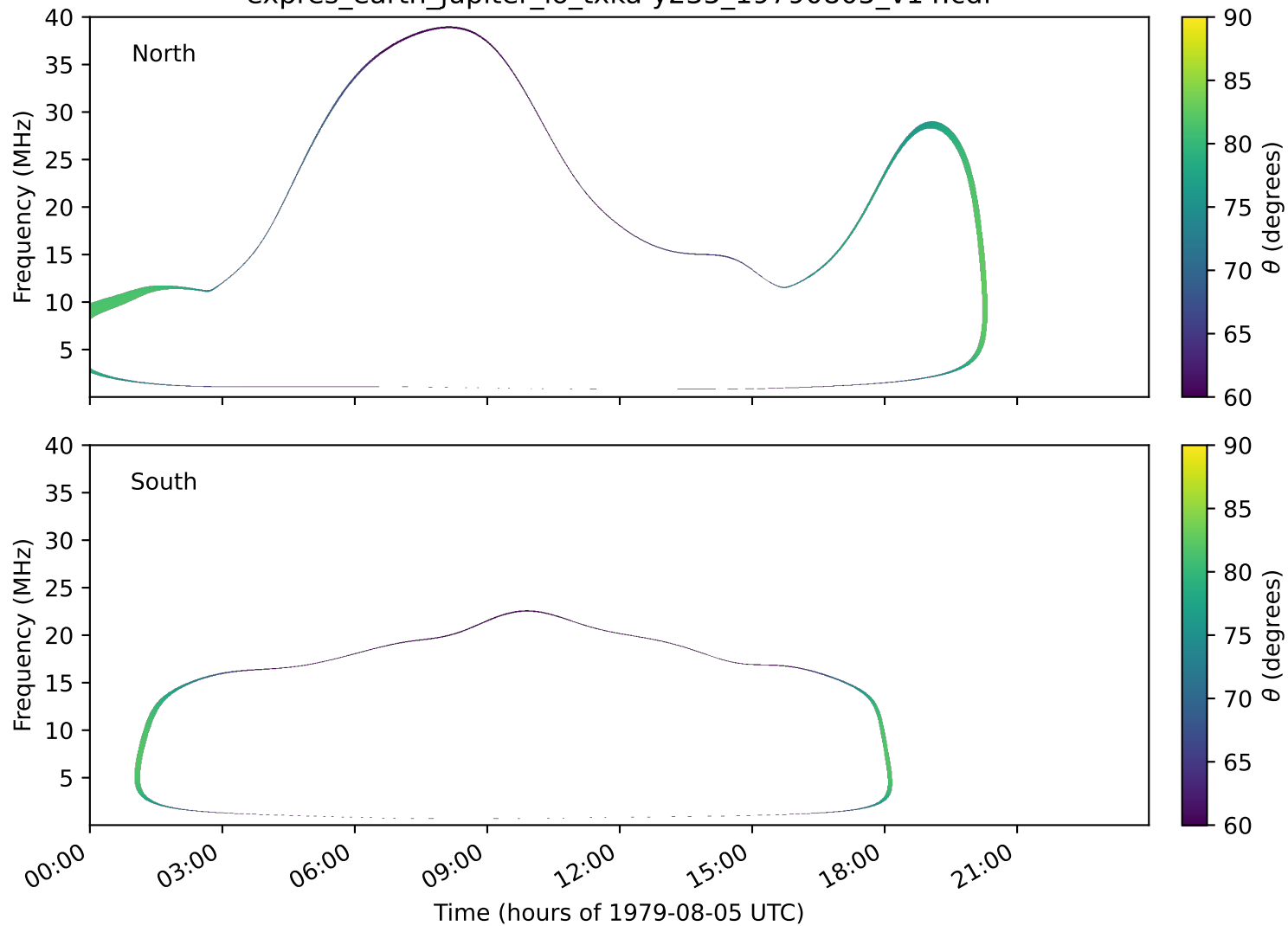
expres_earth_jupiter_io_txka-y235_19790805_v14.cdf
