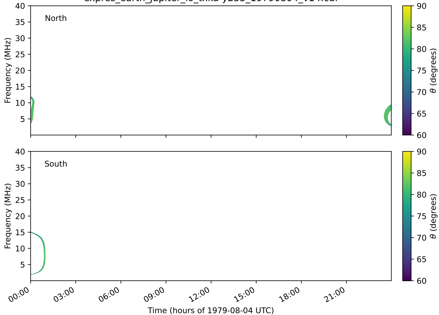
expres_earth_jupiter_io_txka-y235_19790804_v14.cdf
