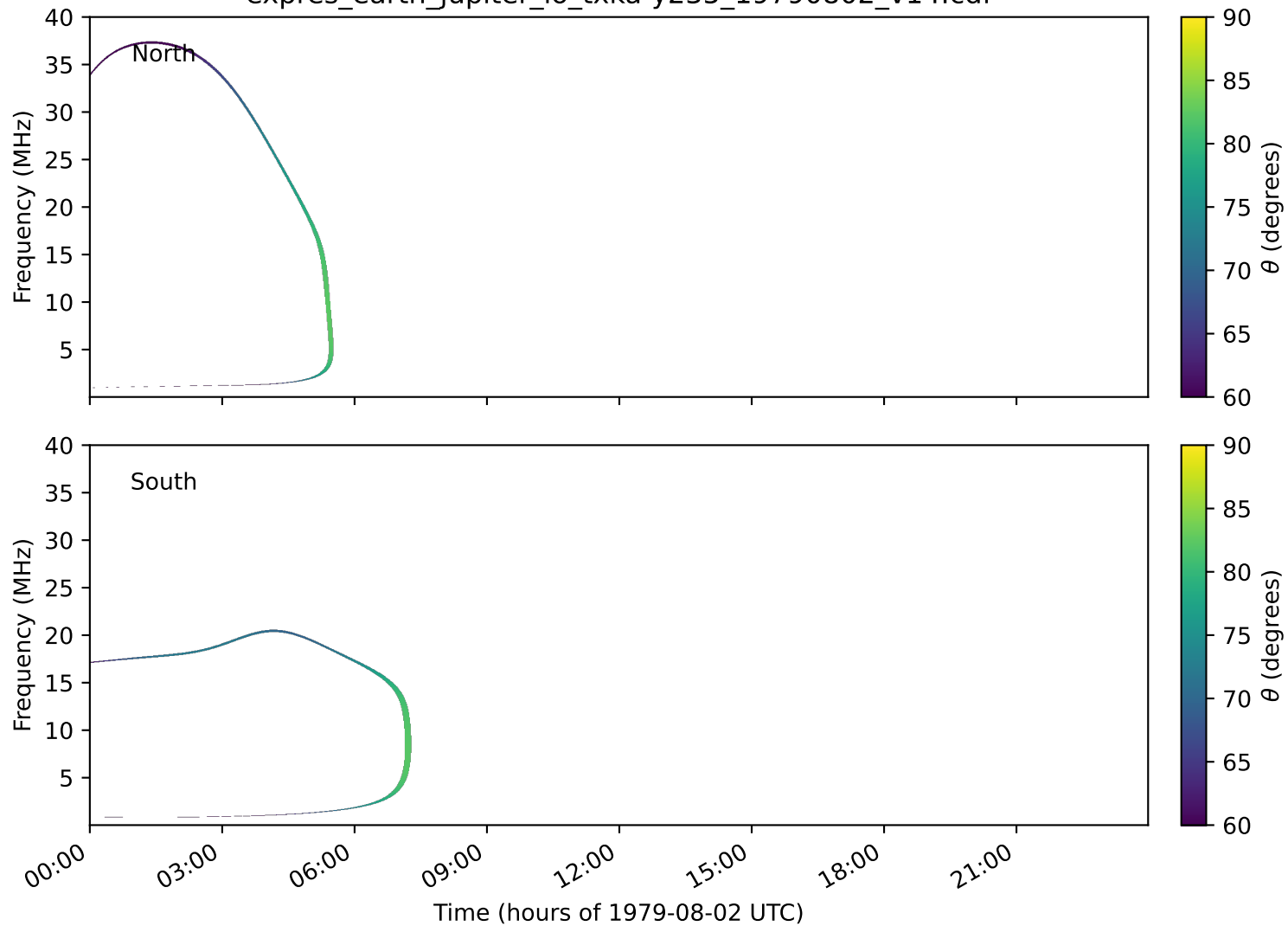
expres_earth_jupiter_io_txka-y235_19790802_v14.cdf
