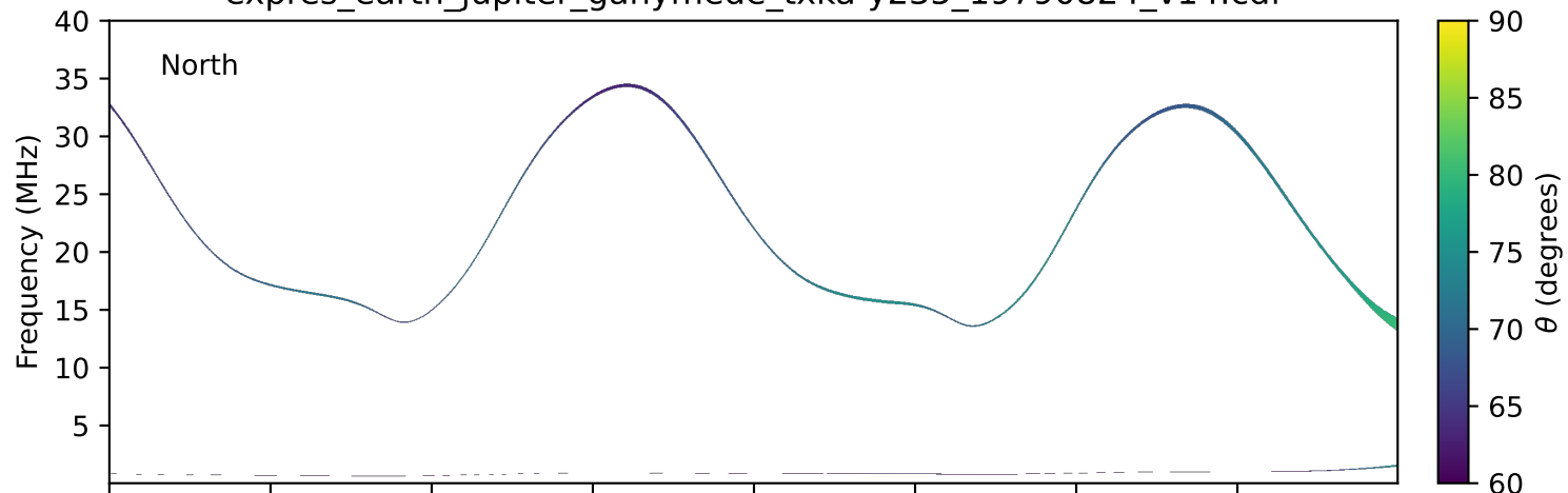
expres_earth_jupiter_ganymede_txka-y235_19790824_v14.cdf
