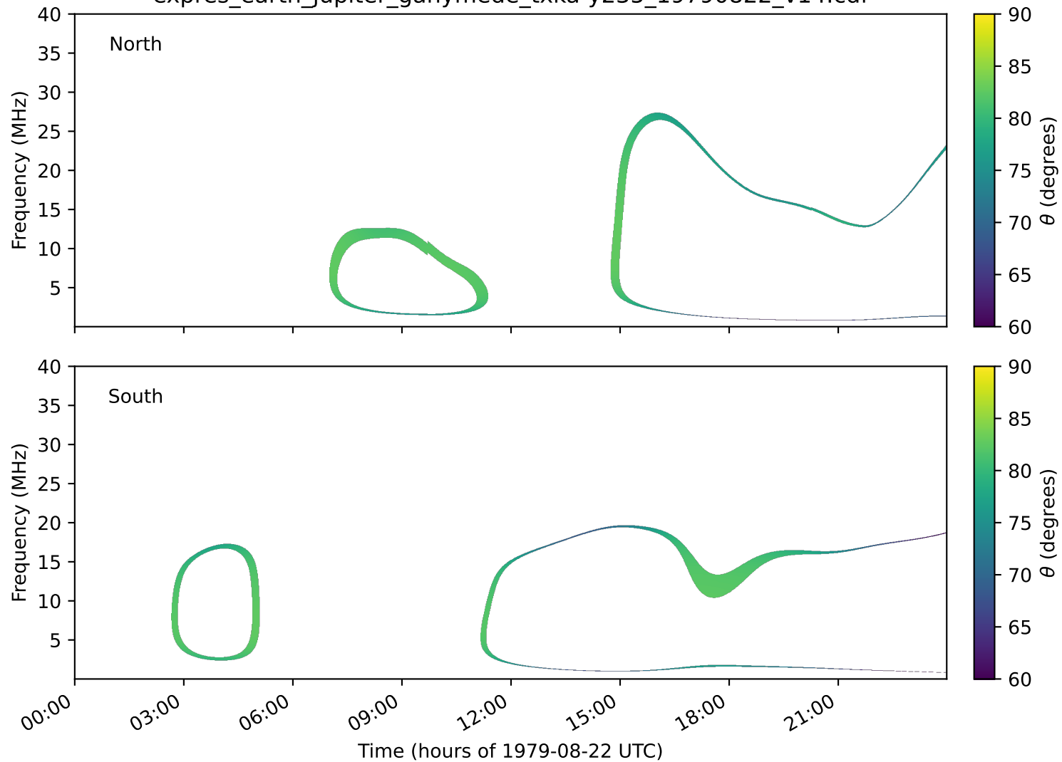
expres_earth_jupiter_ganymede_txka-y235_19790822_v14.cdf
