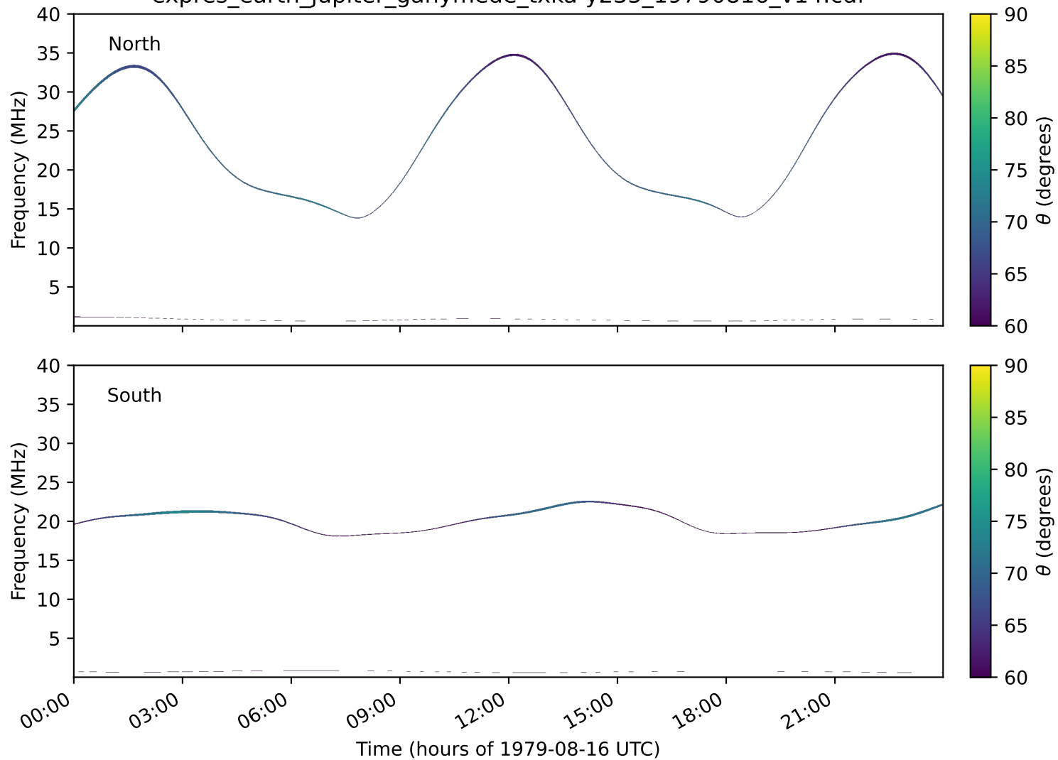
expres_earth_jupiter_ganymede_txka-y235_19790816_v14.cdf
