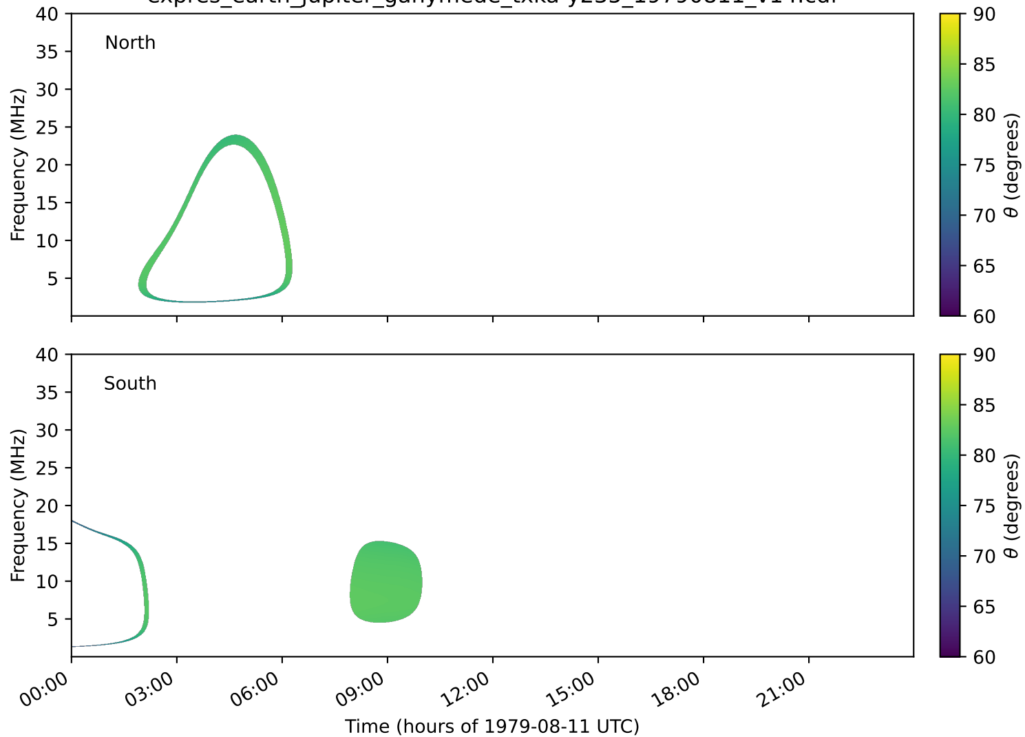
expres_earth_jupiter_ganymede_txka-y235_19790811_v14.cdf
