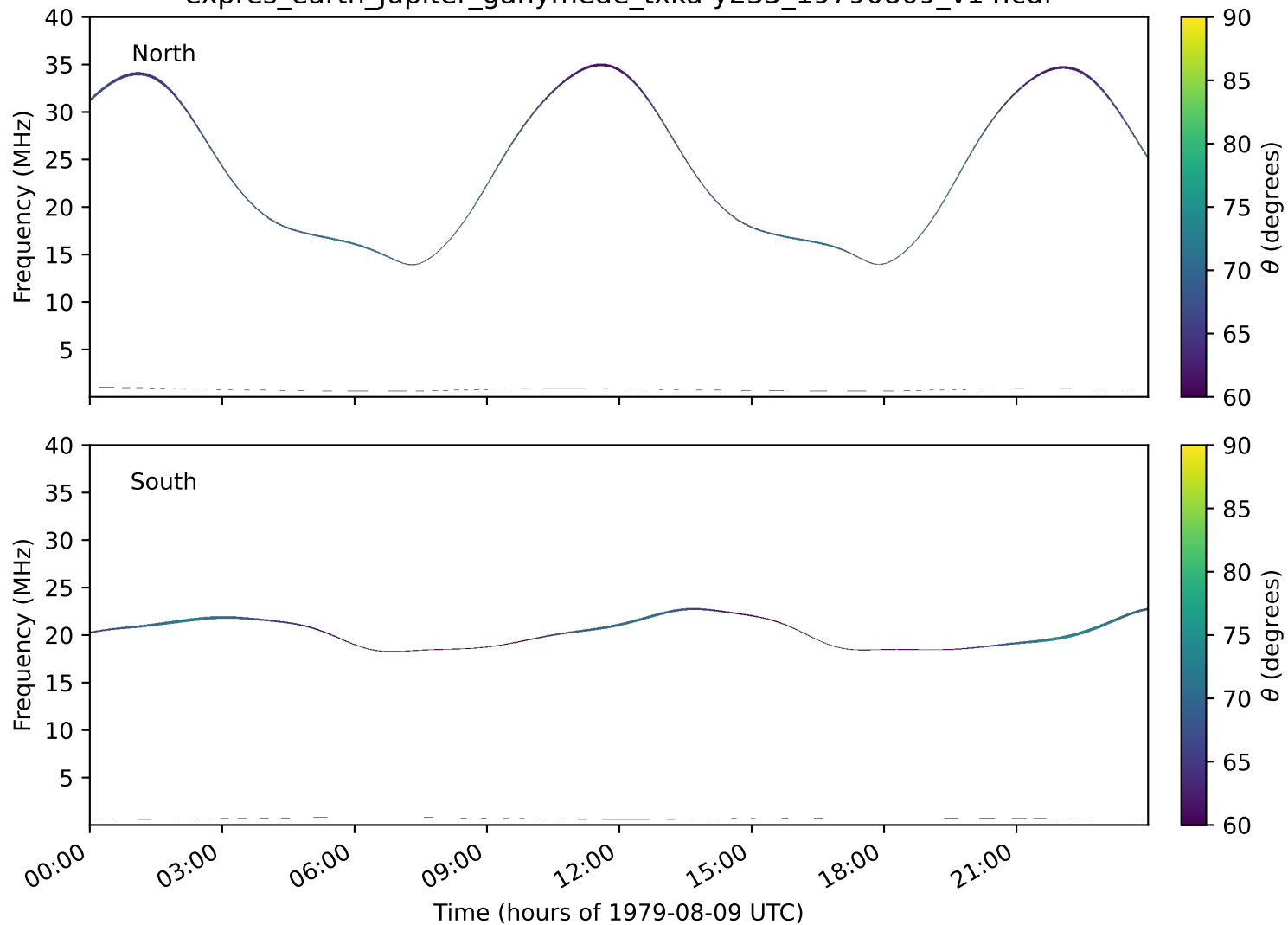
expres_earth_jupiter_ganymede_txka-y235_19790809_v14.cdf
