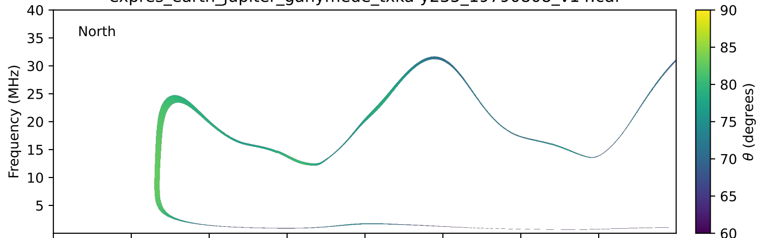
expres_earth_jupiter_ganymede_txka-y235_19790808_v14.cdf
