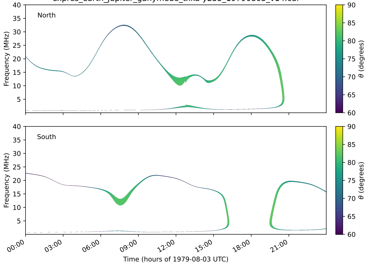
expres_earth_jupiter_ganymede_txka-y235_19790803_v14.cdf
