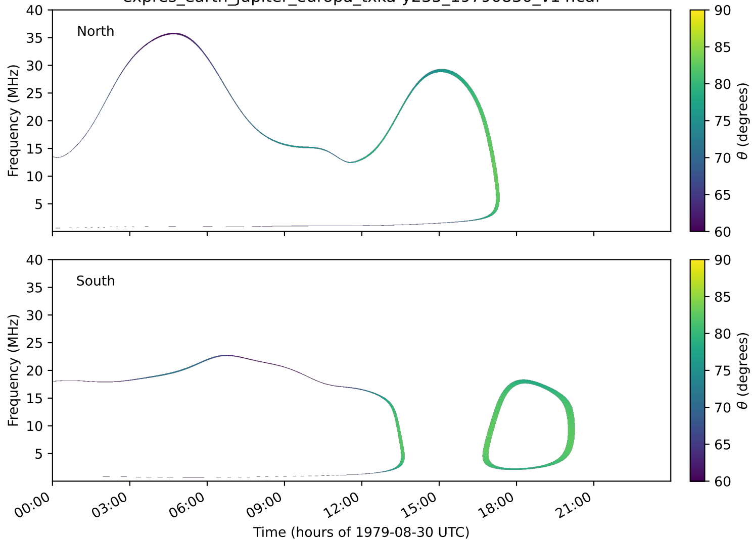
expres_earth_jupiter_europa_txka-y235_19790830_v14.cdf
