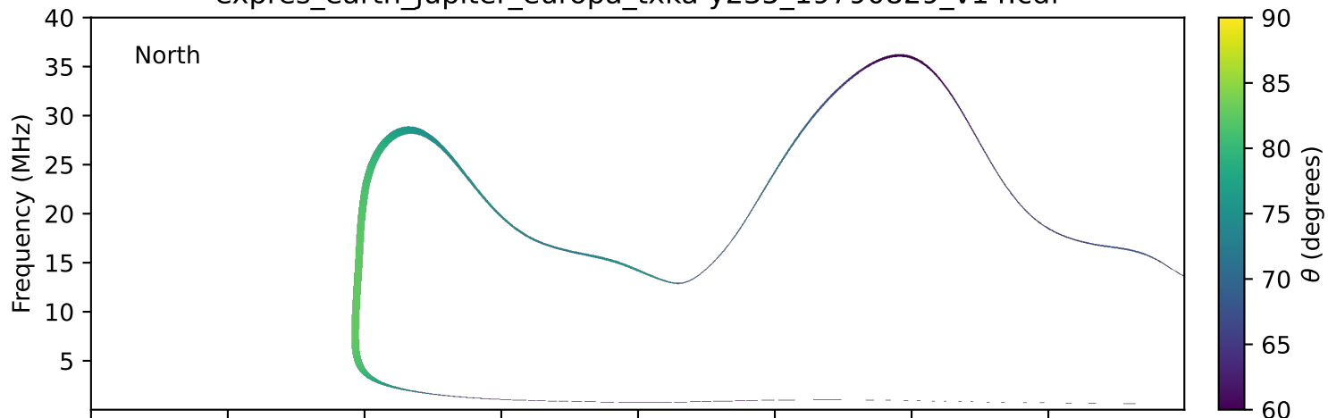
expres_earth_jupiter_europa_txka-y235_19790829_v14.cdf
