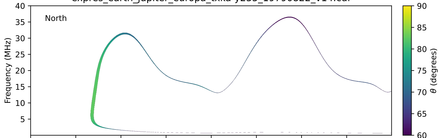
expres_earth_jupiter_europa_txka-y235_19790822_v14.cdf
