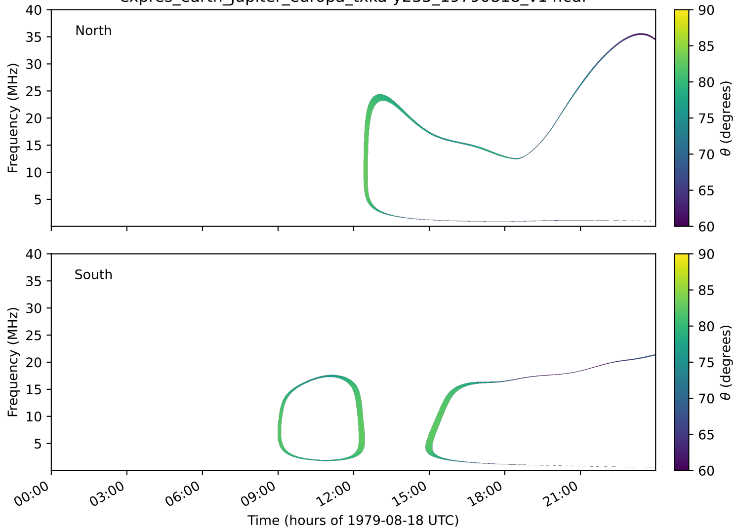
expres_earth_jupiter_europa_txka-y235_19790818_v14.cdf
