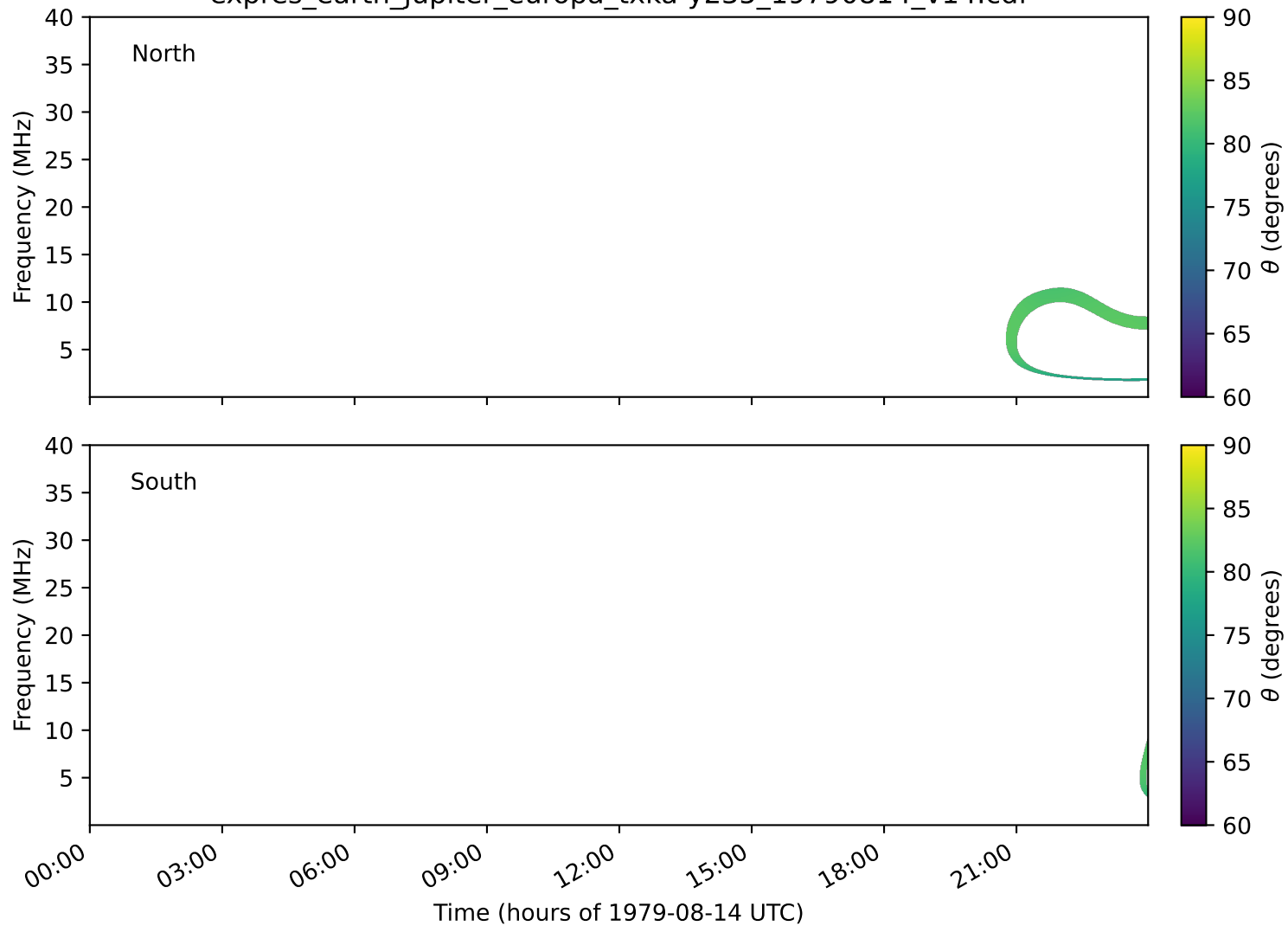
expres_earth_jupiter_europa_txka-y235_19790814_v14.cdf
