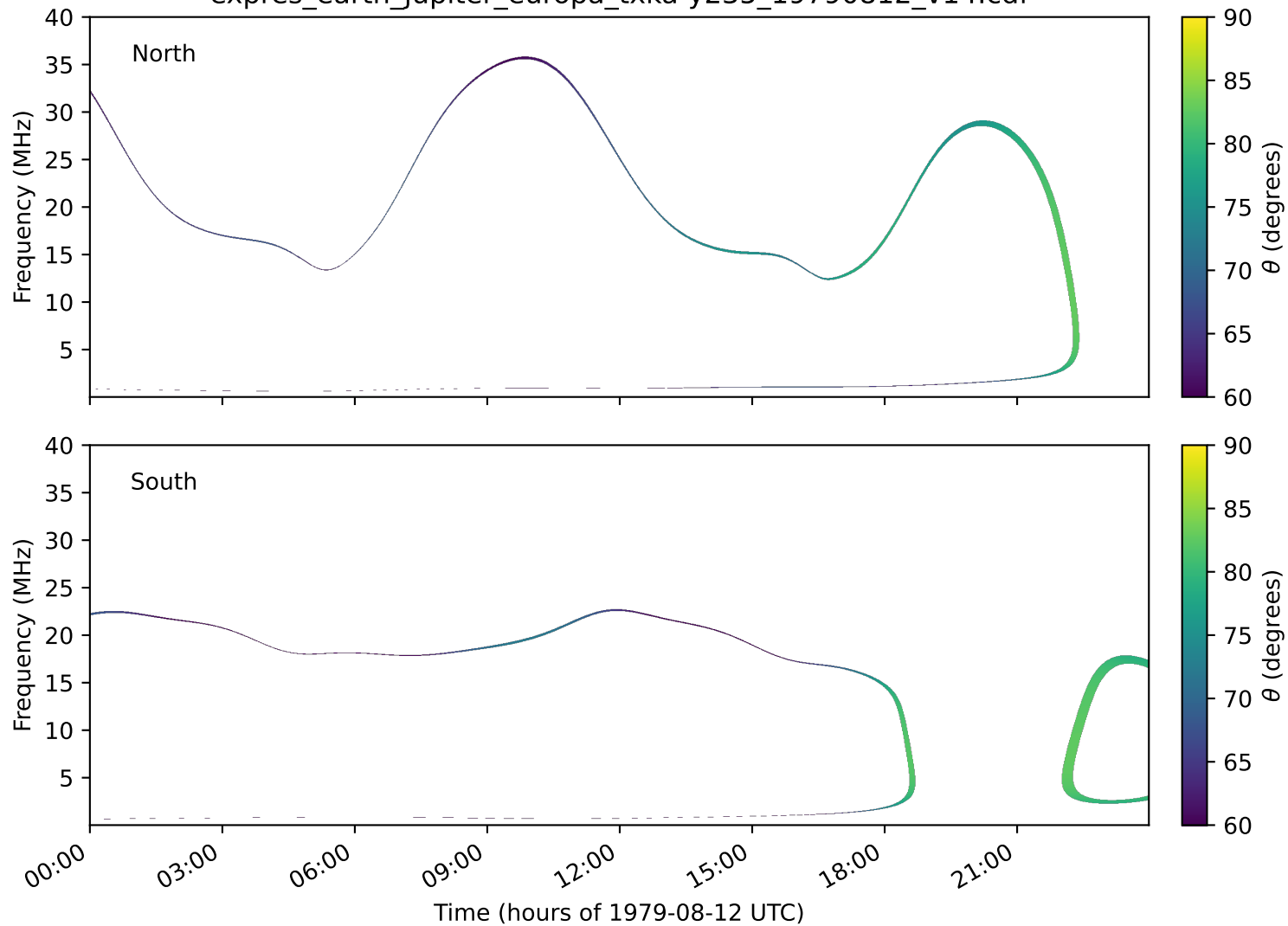
expres_earth_jupiter_europa_txka-y235_19790812_v14.cdf
