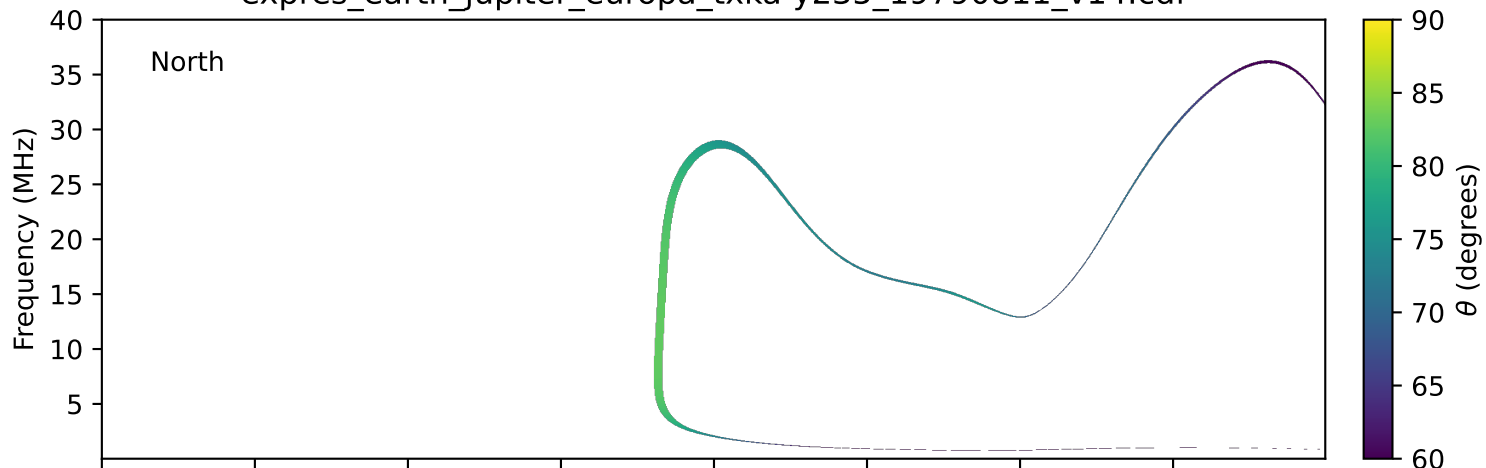
expres_earth_jupiter_europa_txka-y235_19790811_v14.cdf
