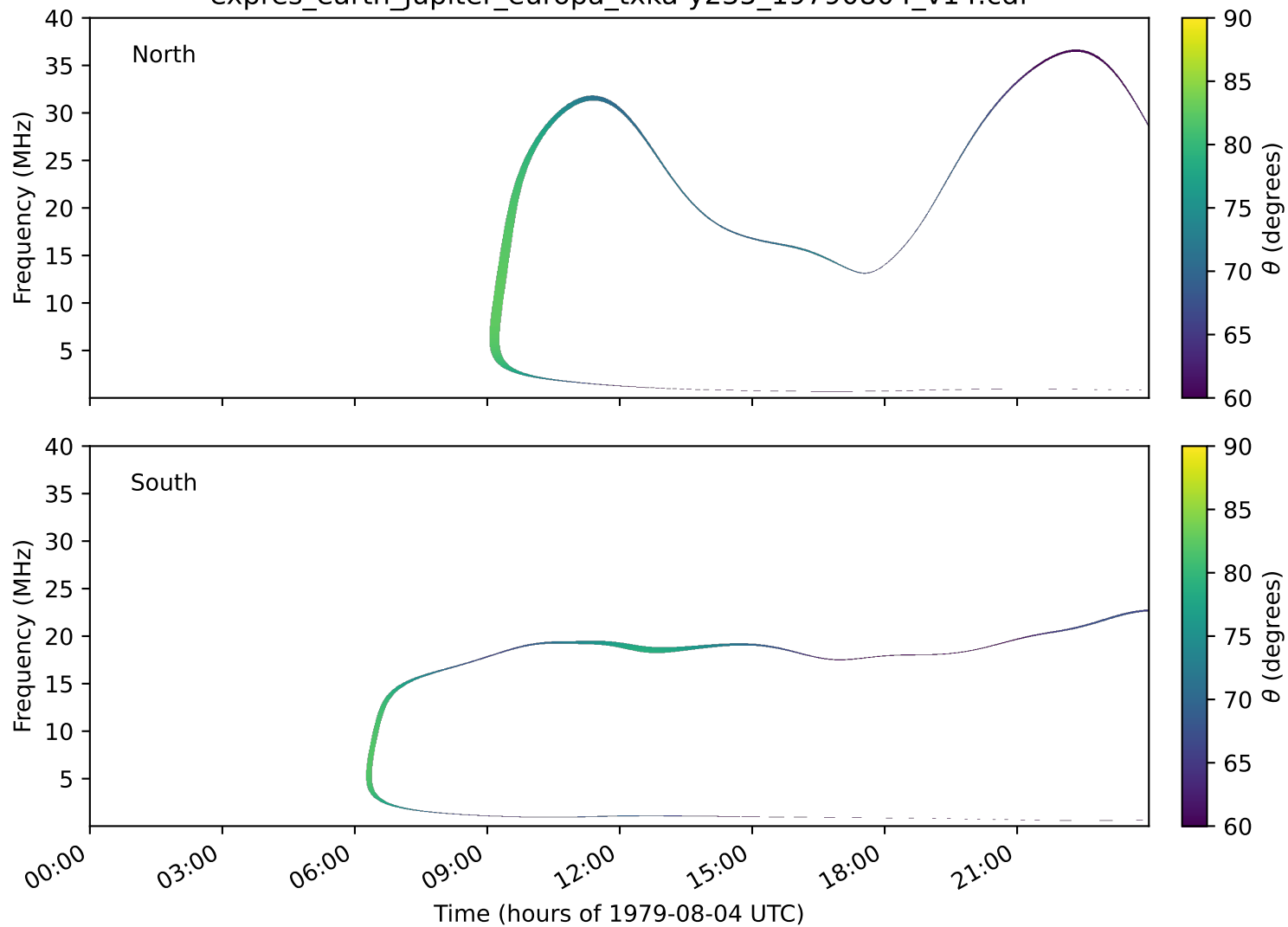
expres_earth_jupiter_europa_txka-y235_19790804_v14.cdf
