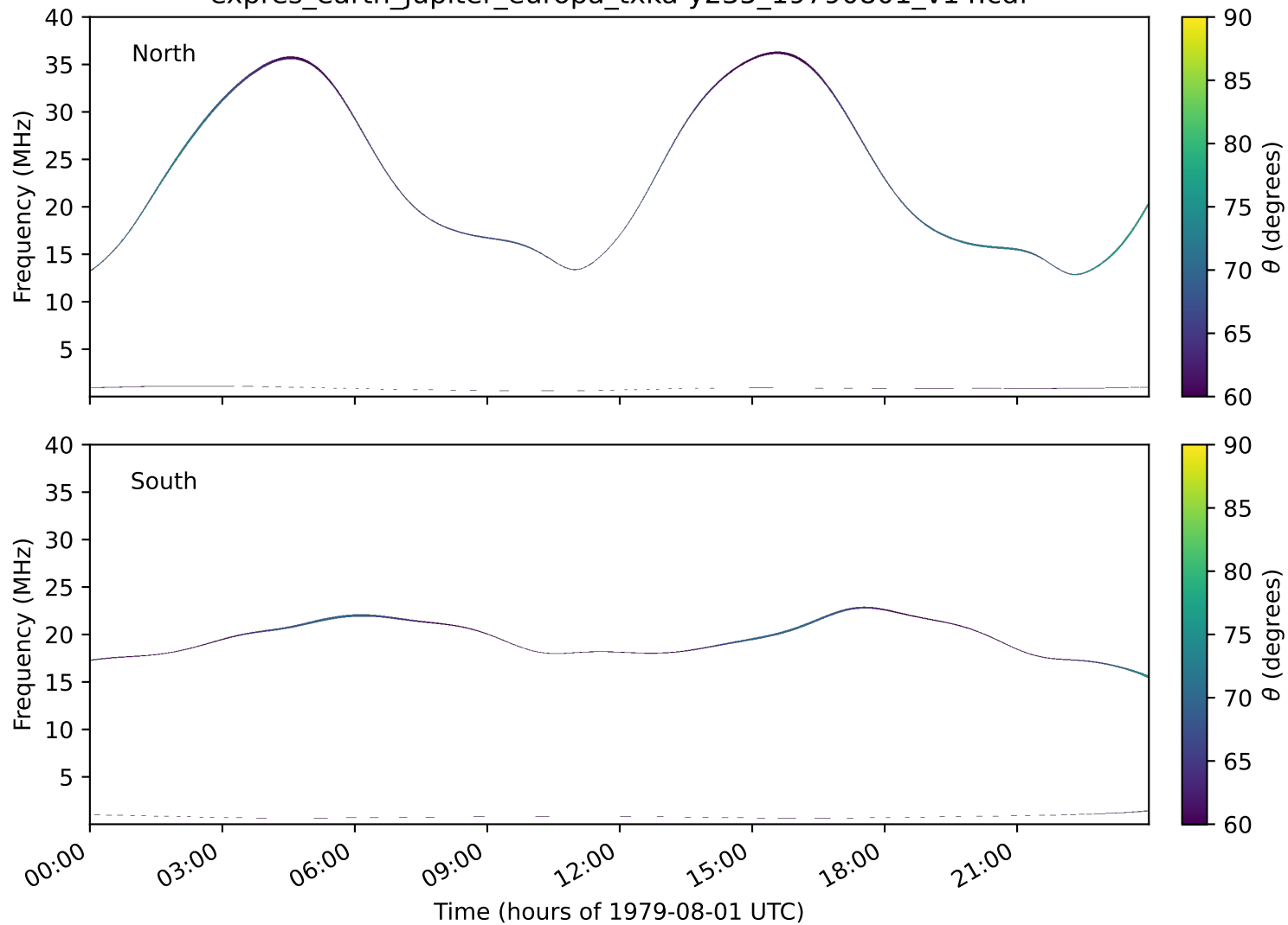
expres_earth_jupiter_europa_txka-y235_19790801_v14.cdf
