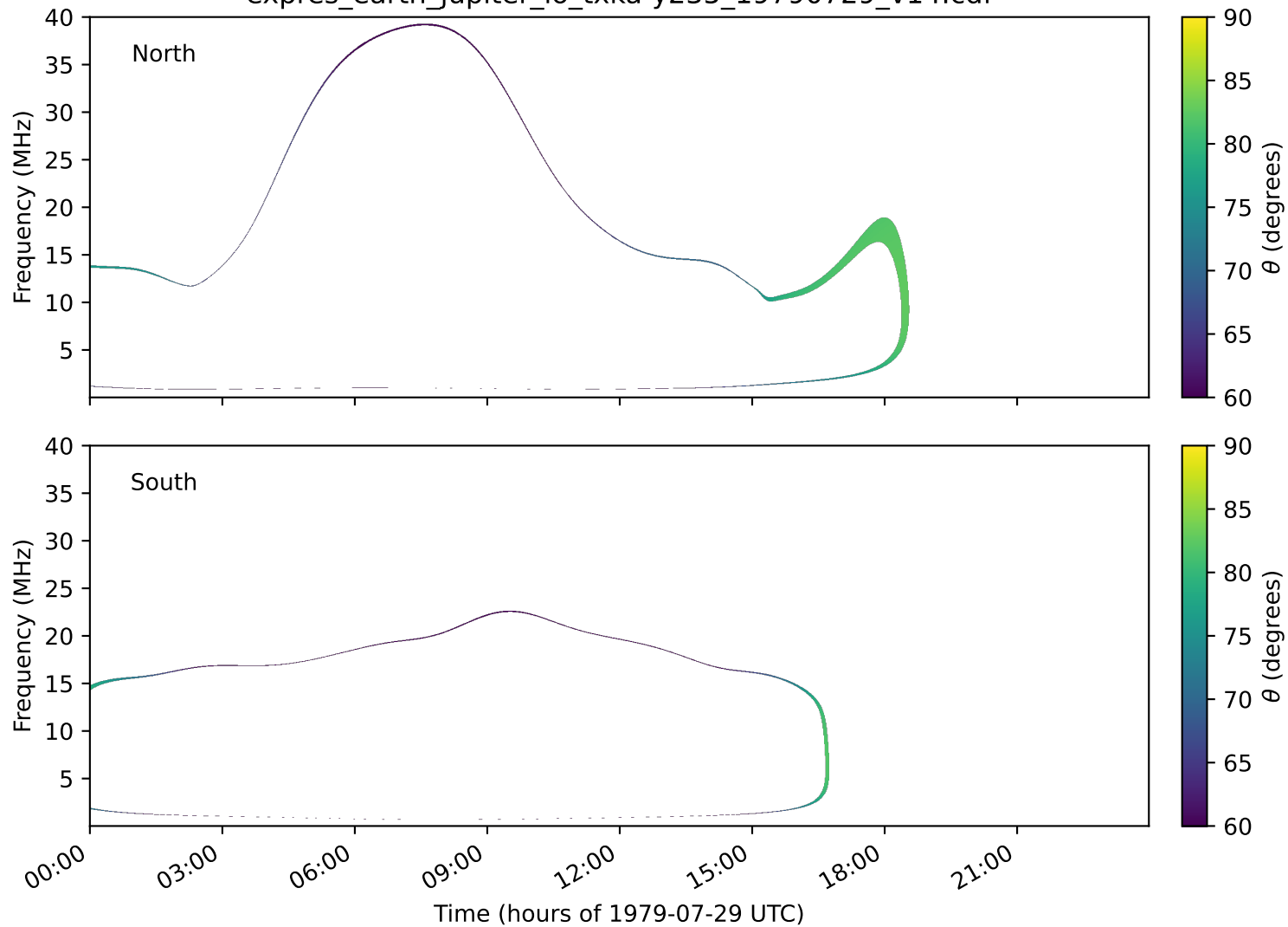
expres_earth_jupiter_io_txka-y235_19790729_v14.cdf
