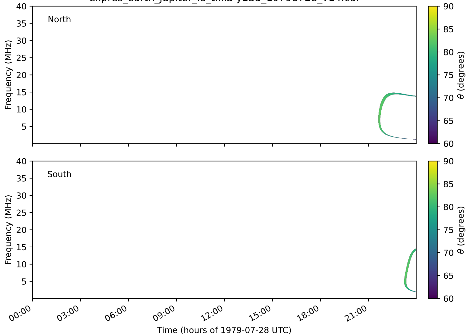
expres_earth_jupiter_io_txka-y235_19790728_v14.cdf
