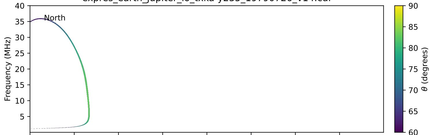
expres_earth_jupiter_io_txka-y235_19790726_v14.cdf
