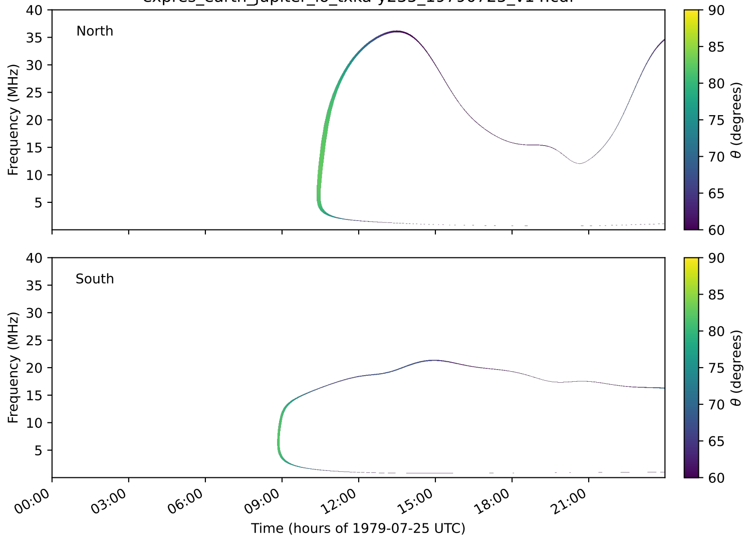
expres_earth_jupiter_io_txka-y235_19790725_v14.cdf
