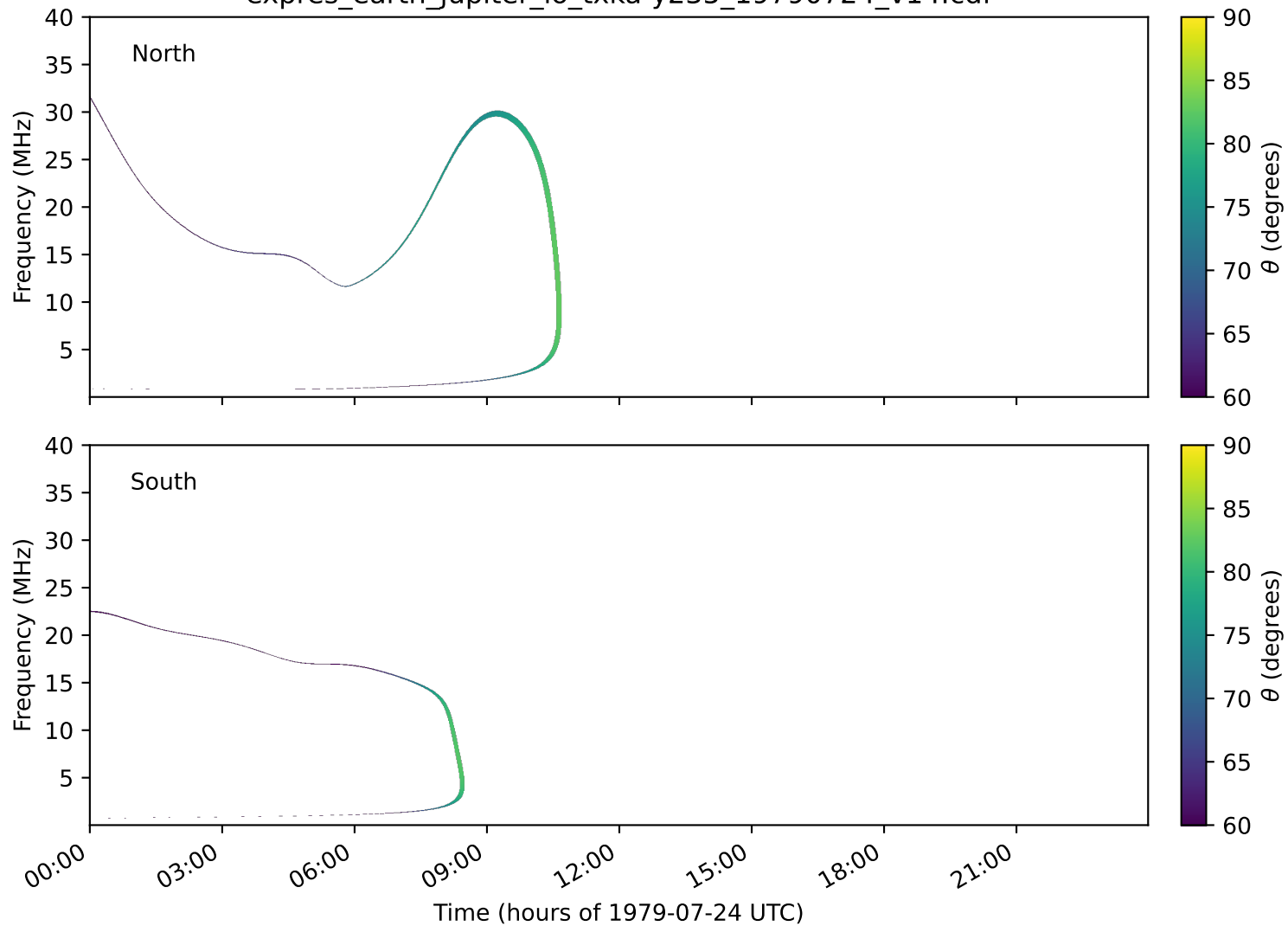
expres_earth_jupiter_io_txka-y235_19790724_v14.cdf
