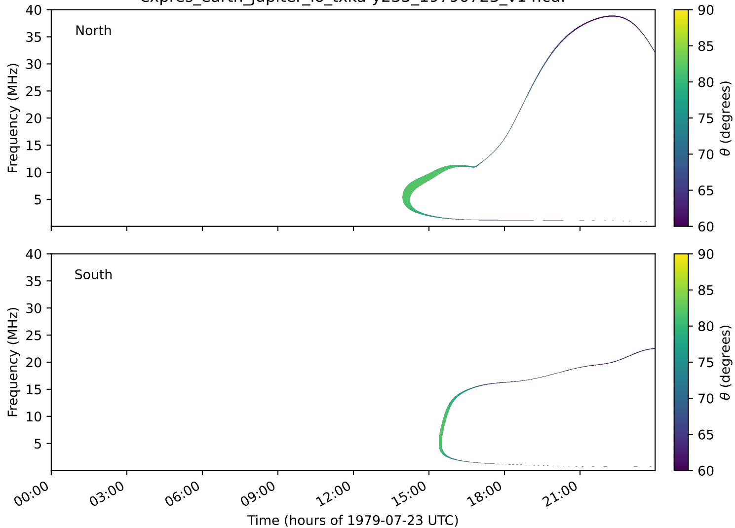
expres_earth_jupiter_io_txka-y235_19790723_v14.cdf
