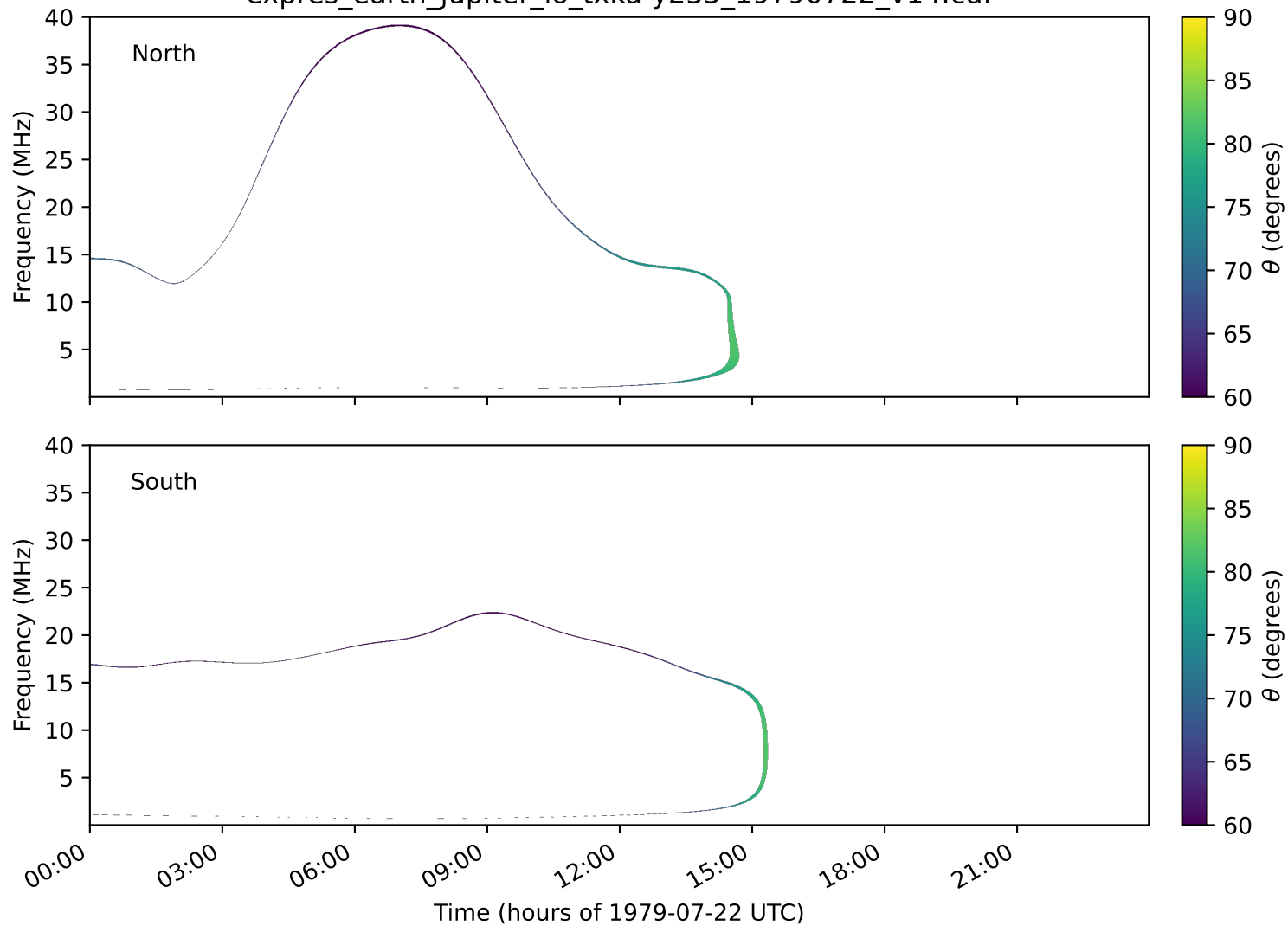
expres_earth_jupiter_io_txka-y235_19790722_v14.cdf
