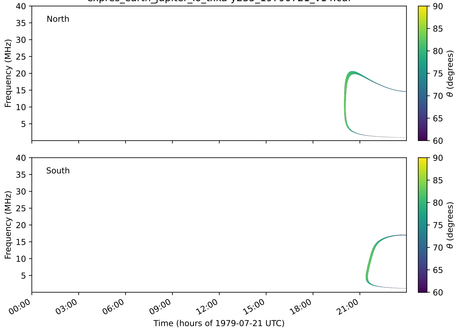
expres_earth_jupiter_io_txka-y235_19790721_v14.cdf
