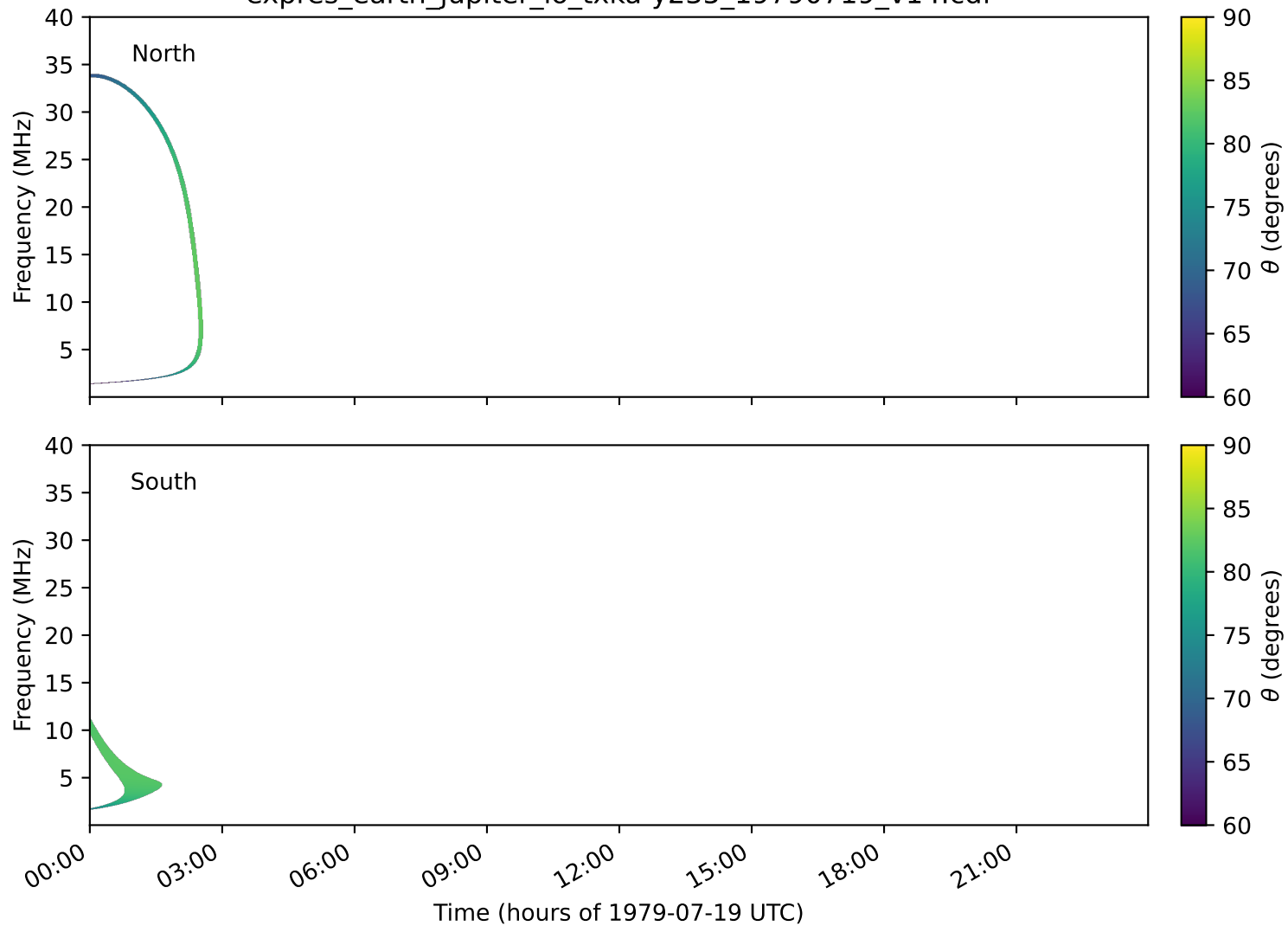
expres_earth_jupiter_io_txka-y235_19790719_v14.cdf
