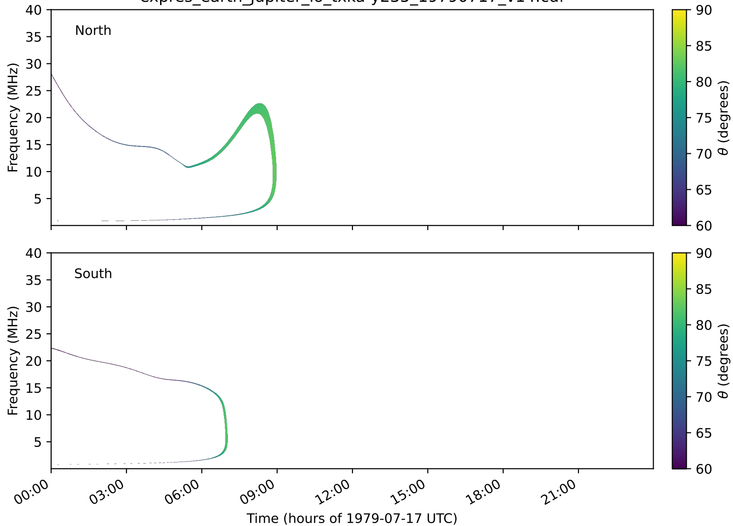
expres_earth_jupiter_io_txka-y235_19790717_v14.cdf
