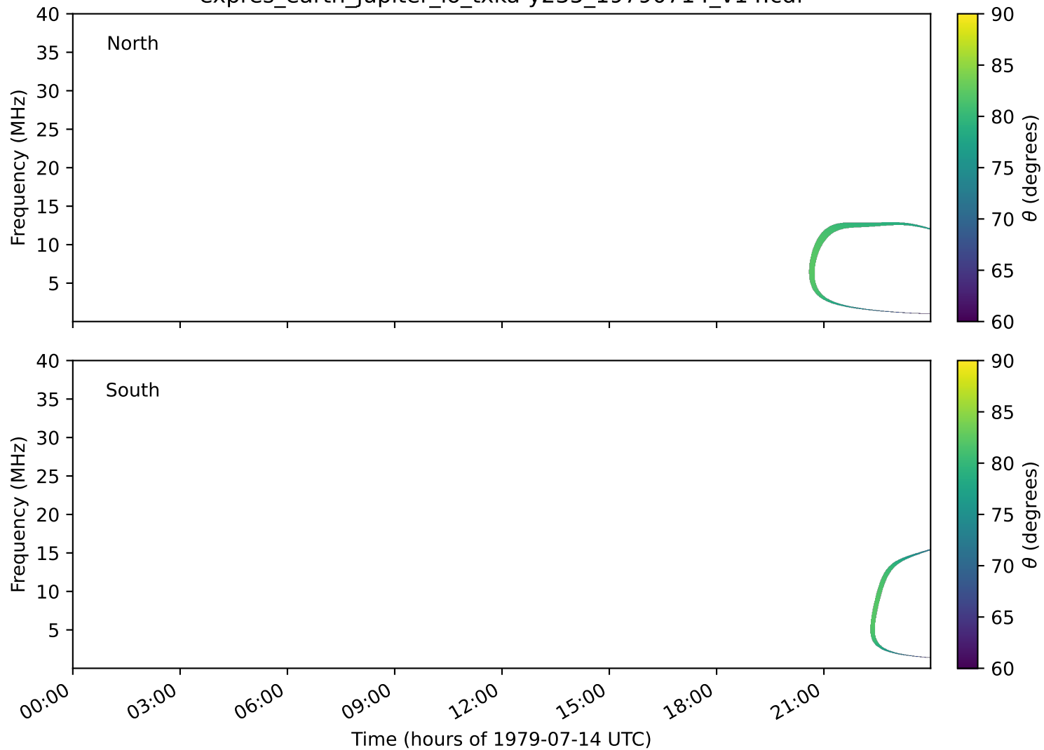
expres_earth_jupiter_io_txka-y235_19790714_v14.cdf
