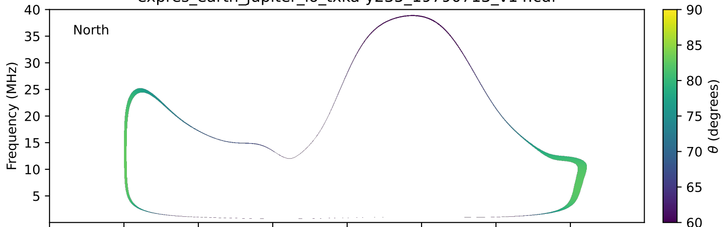
expres_earth_jupiter_io_txka-y235_19790713_v14.cdf
