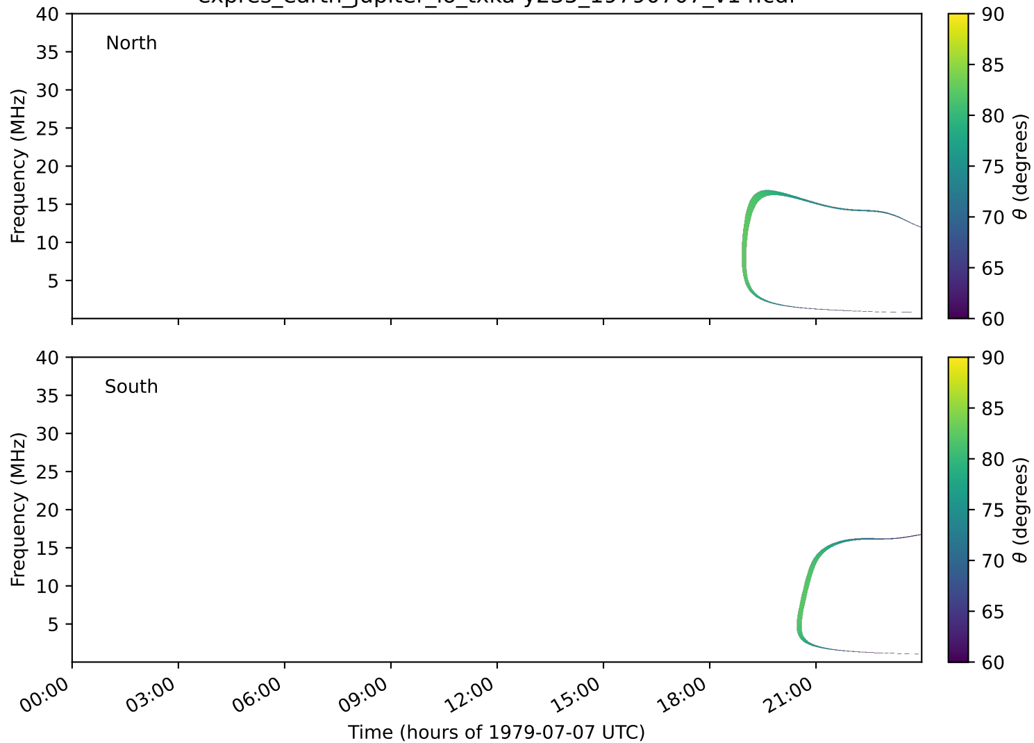
expres_earth_jupiter_io_txka-y235_19790707_v14.cdf
