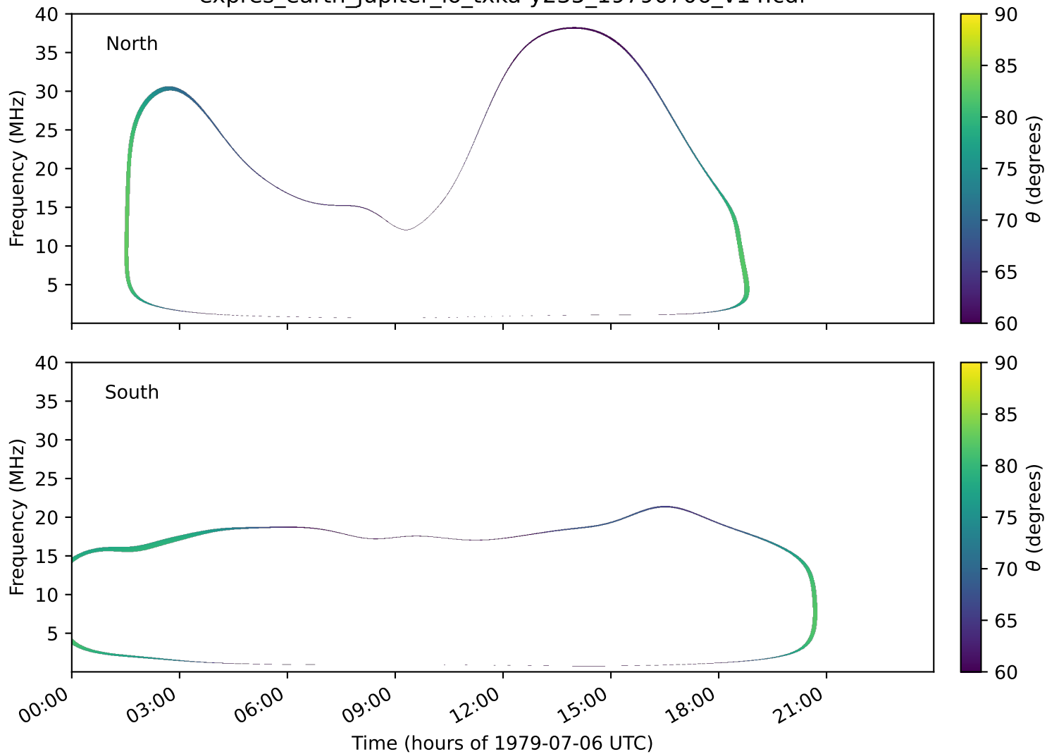
expres_earth_jupiter_io_txka-y235_19790706_v14.cdf
