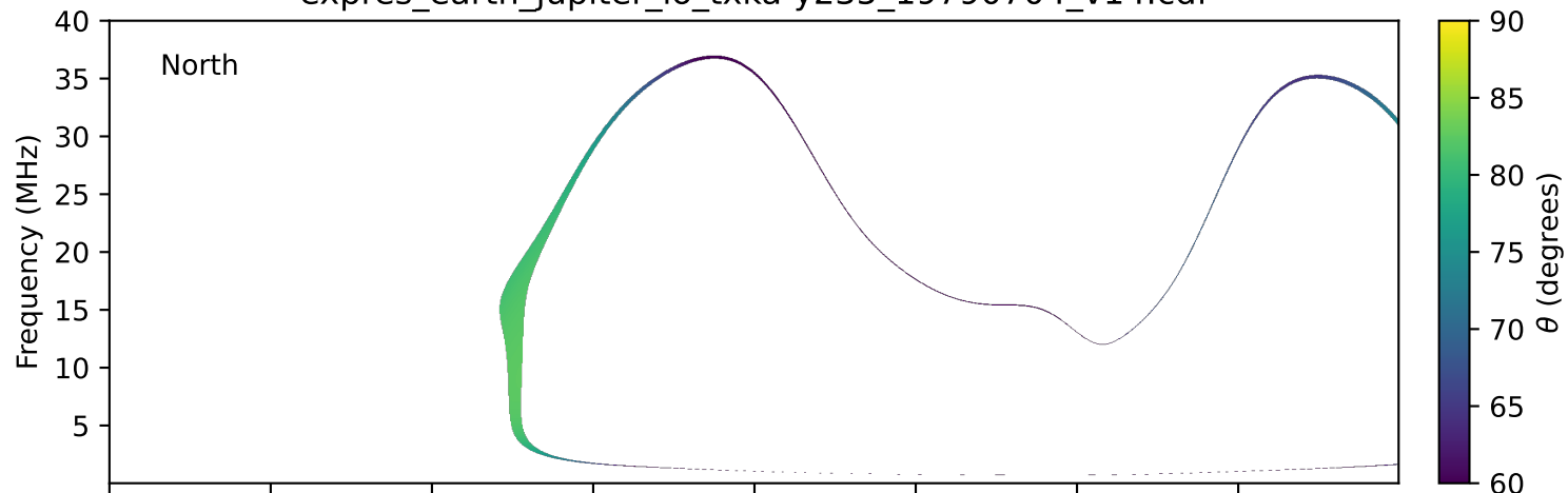
expres_earth_jupiter_io_txka-y235_19790704_v14.cdf
