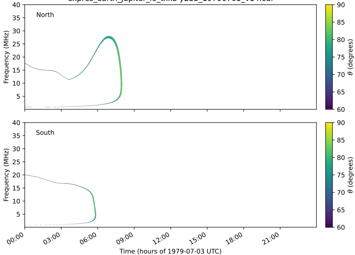
expres_earth_jupiter_io_txka-y235_19790703_v14.cdf
