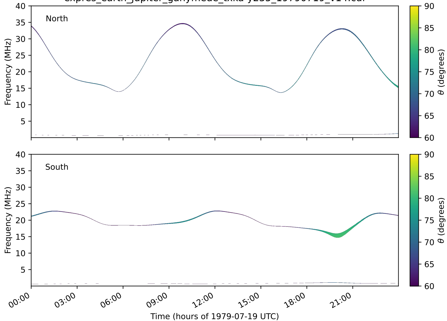
expres_earth_jupiter_ganymede_txka-y235_19790719_v14.cdf
