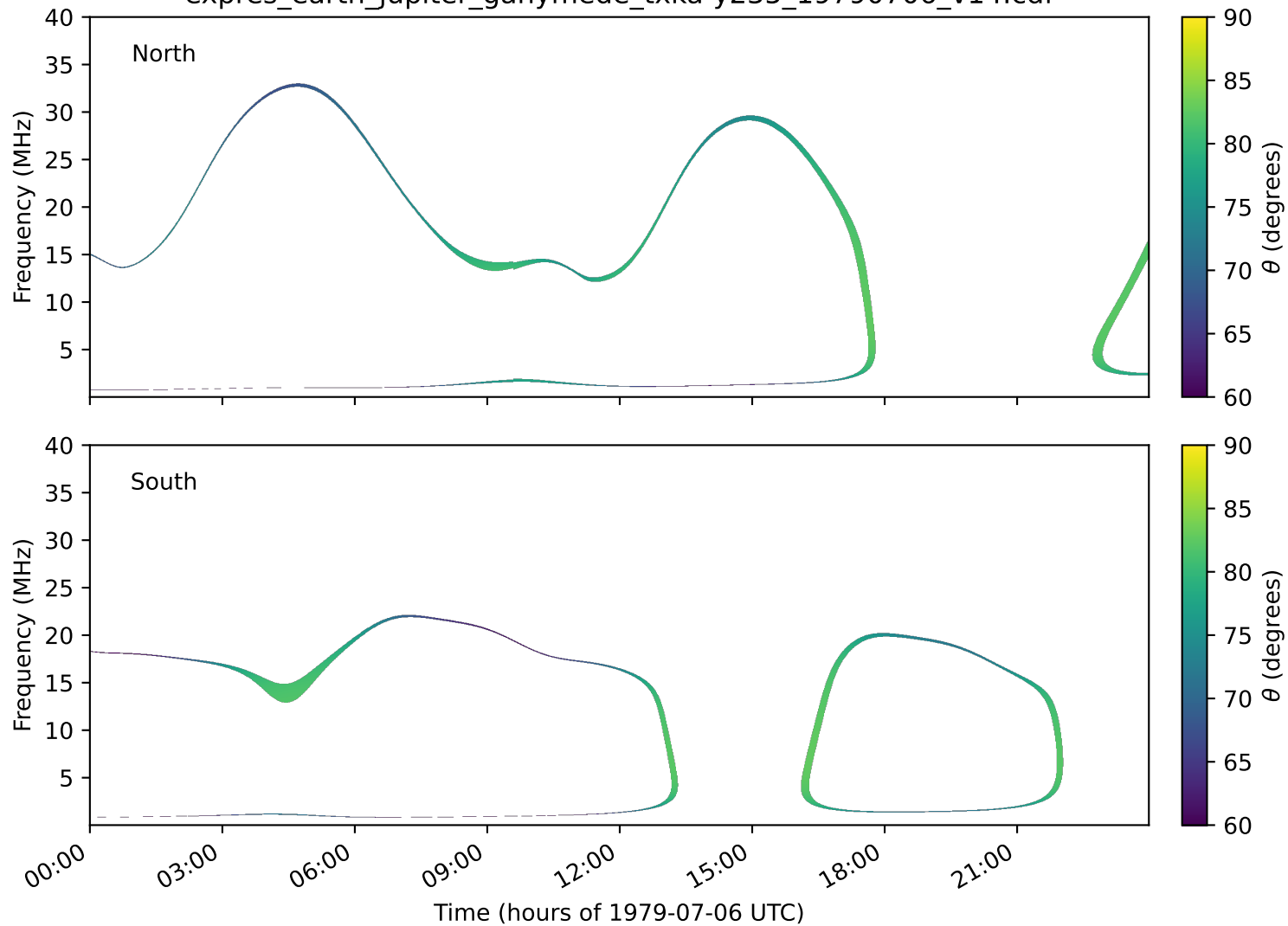
expres_earth_jupiter_ganymede_txka-y235_19790706_v14.cdf
