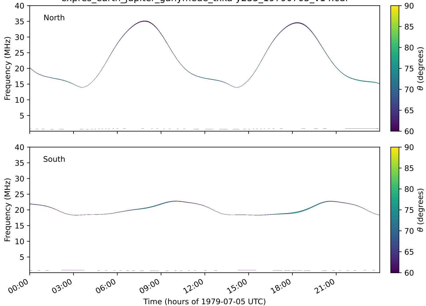
expres_earth_jupiter_ganymede_txka-y235_19790705_v14.cdf
