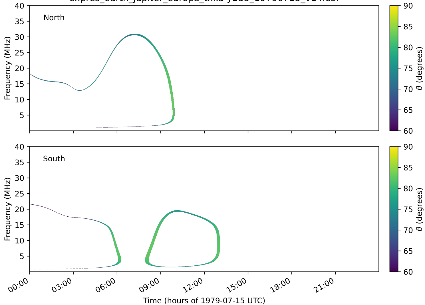
expres_earth_jupiter_europa_txka-y235_19790715_v14.cdf
