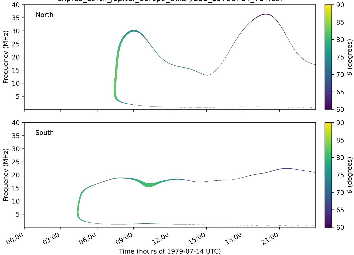
expres_earth_jupiter_europa_txka-y235_19790714_v14.cdf
