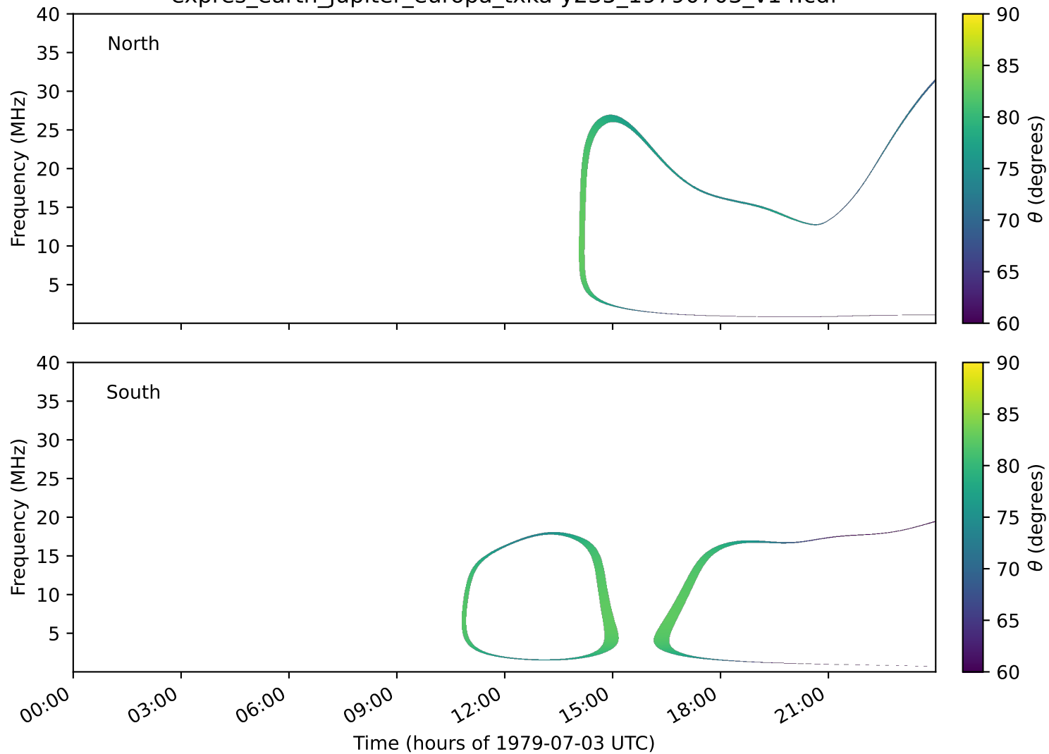
expres_earth_jupiter_europa_txka-y235_19790703_v14.cdf
