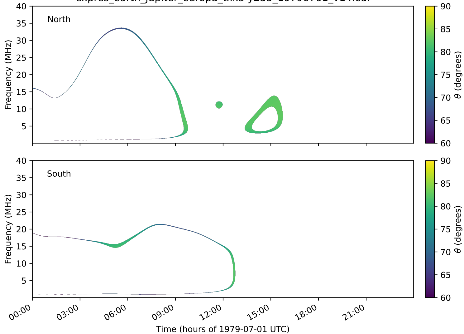
expres_earth_jupiter_europa_txka-y235_19790701_v14.cdf
