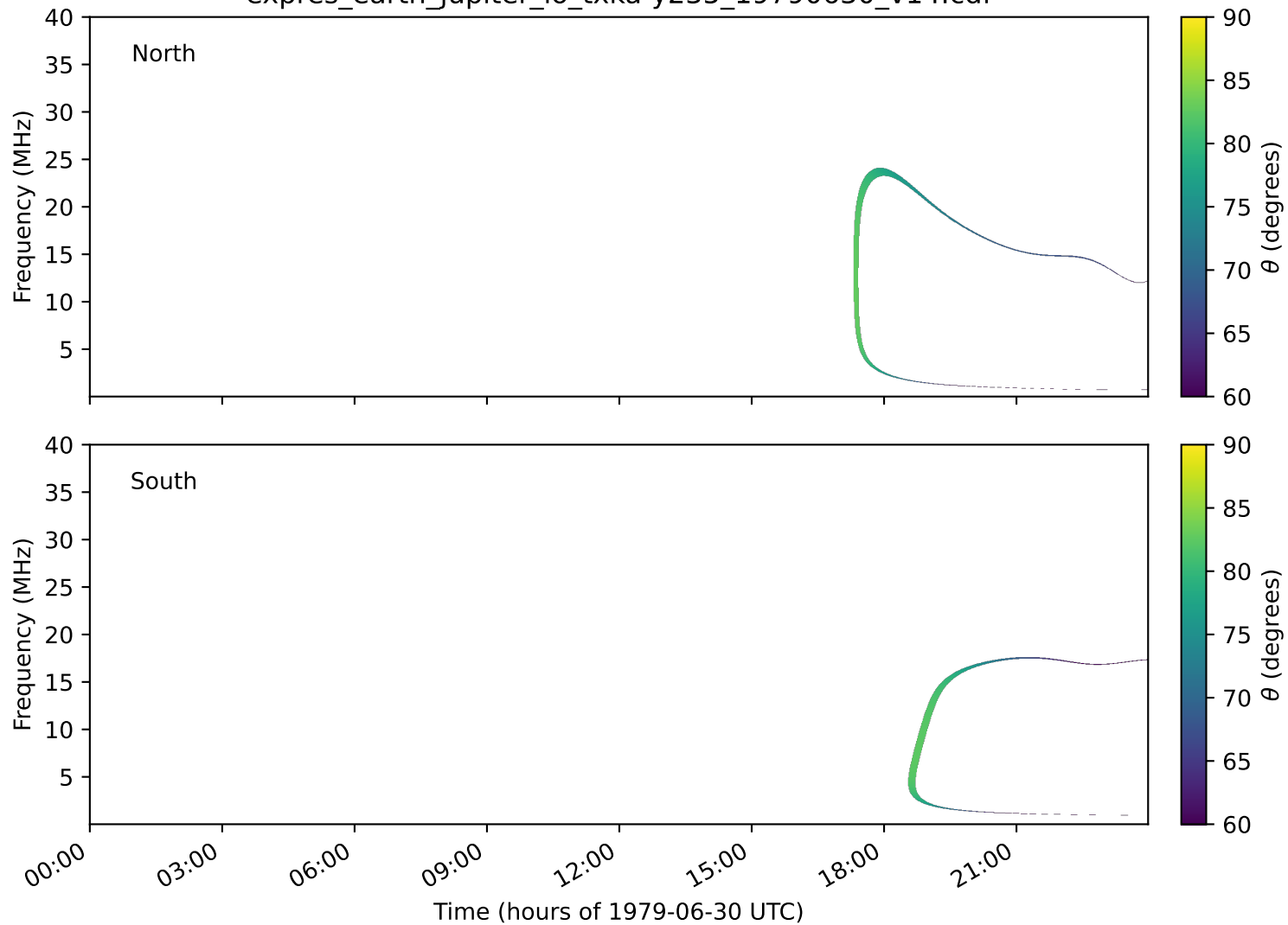
expres_earth_jupiter_io_txka-y235_19790630_v14.cdf
