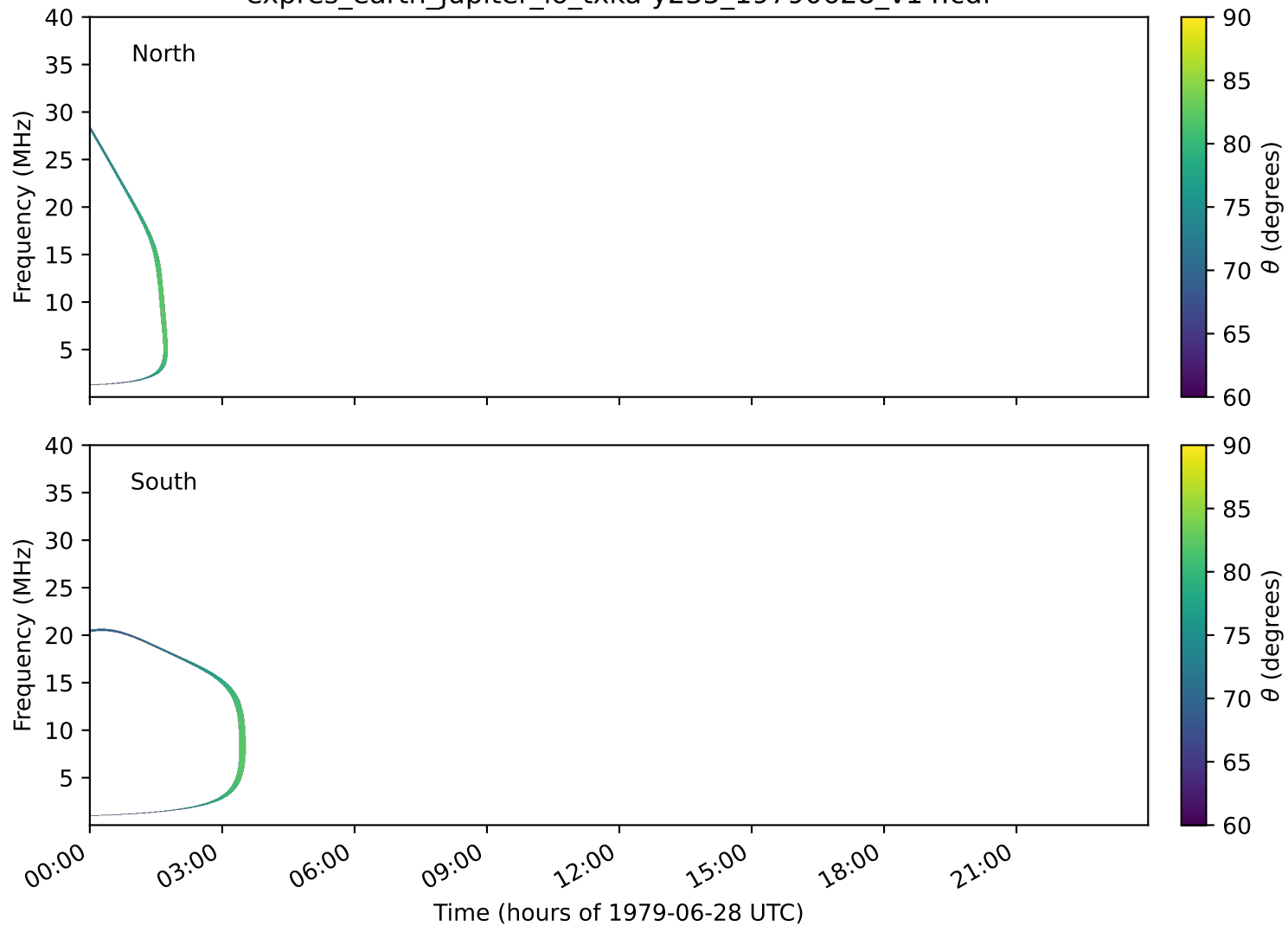
expres_earth_jupiter_io_txka-y235_19790628_v14.cdf
