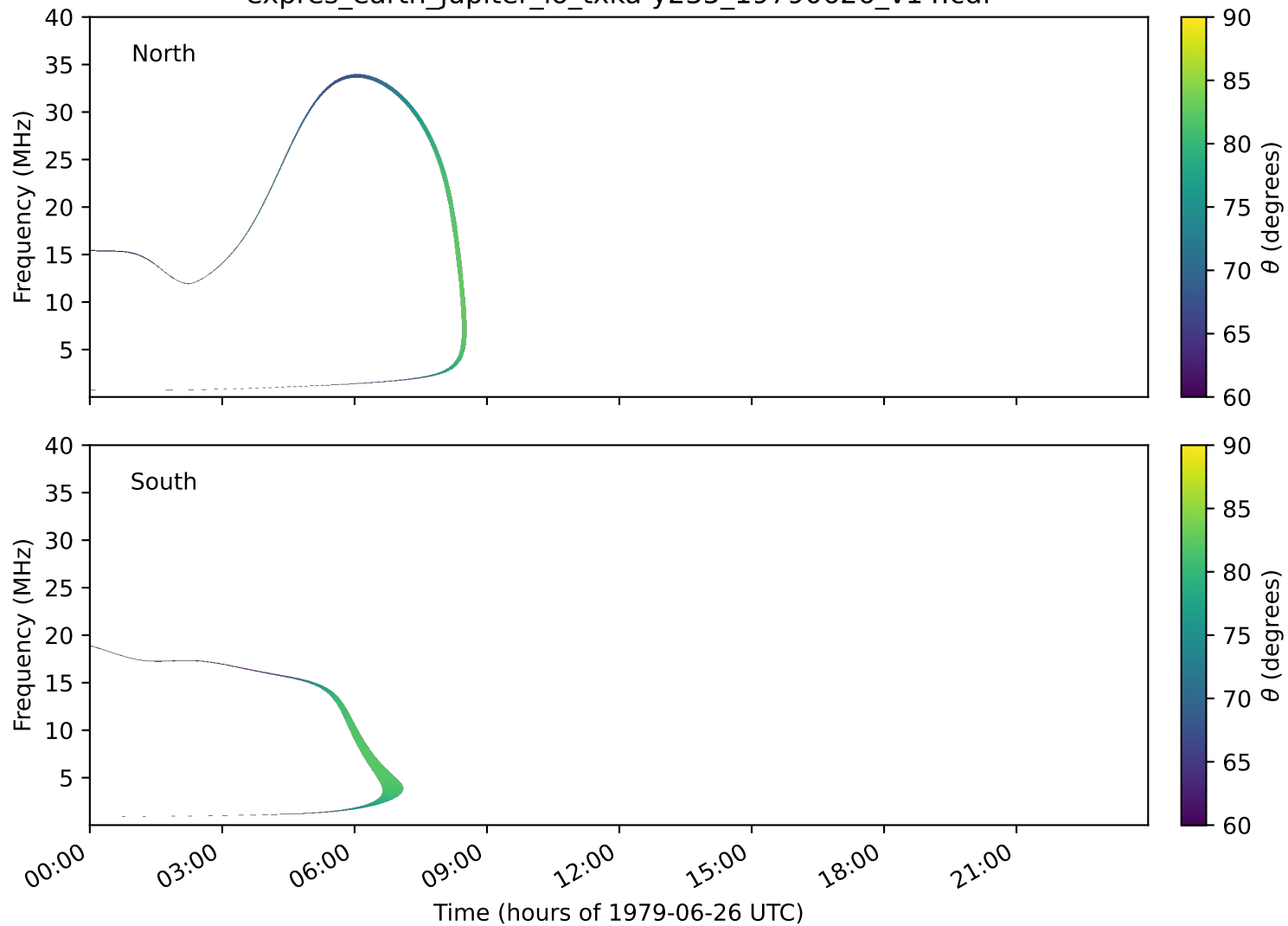
expres_earth_jupiter_io_txka-y235_19790626_v14.cdf
