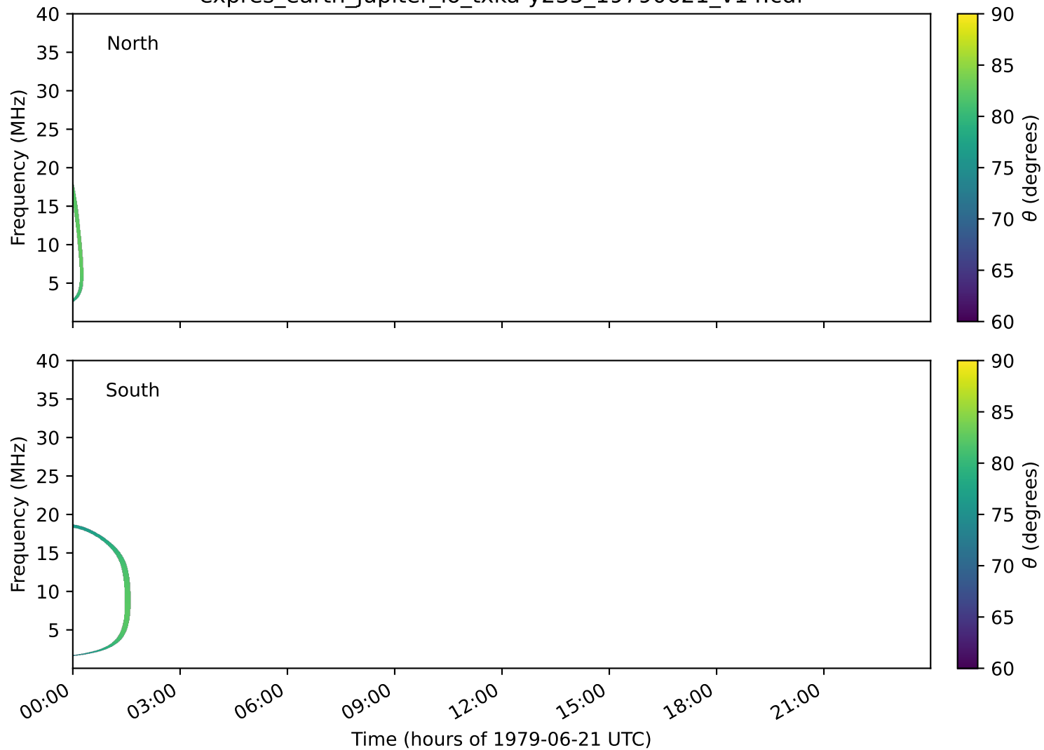
expres_earth_jupiter_io_txka-y235_19790621_v14.cdf
